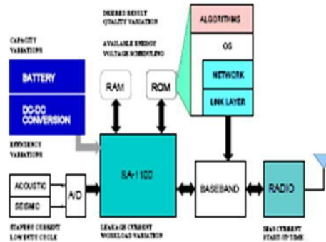
Figure 1. Architectural view of microsensor node
