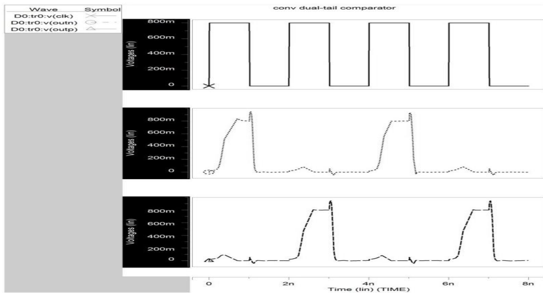
Fig. 9: Simulated Waveform of Comparator 1 (180nm)
