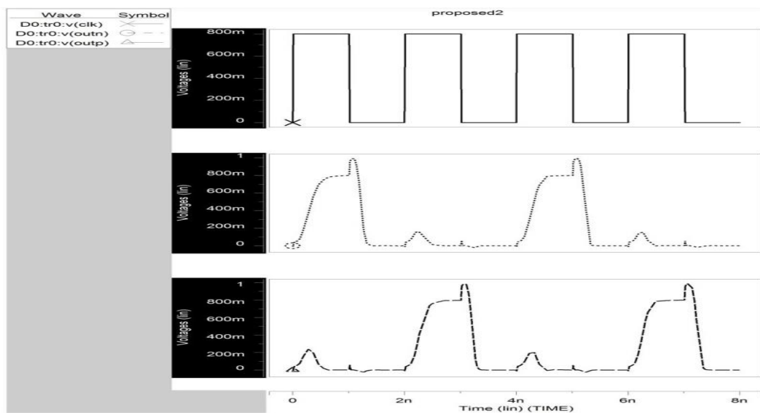
Fig. 11: Simulated Waveform of Comparator 3 (180nm)
