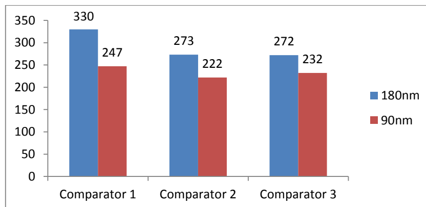
Fig. 16: Delay comparison of dynamic comparators
