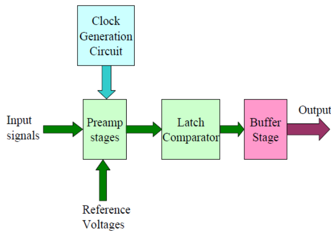
Fig. 1: High Speed Comparator Architecture
