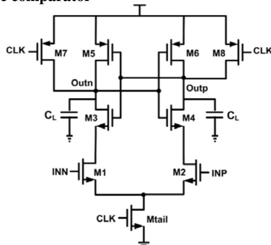
Fig. 4: Conventional Dynamic Comparator (Comparator 1)
