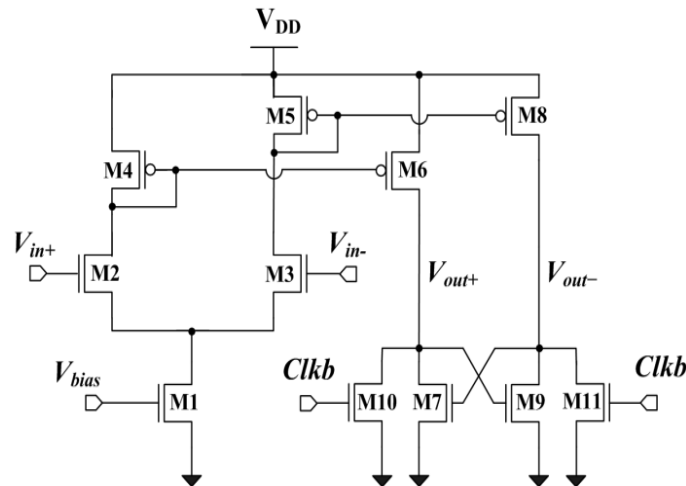
Fig. 3: Pre-Amplifier Based Latched Comparator
