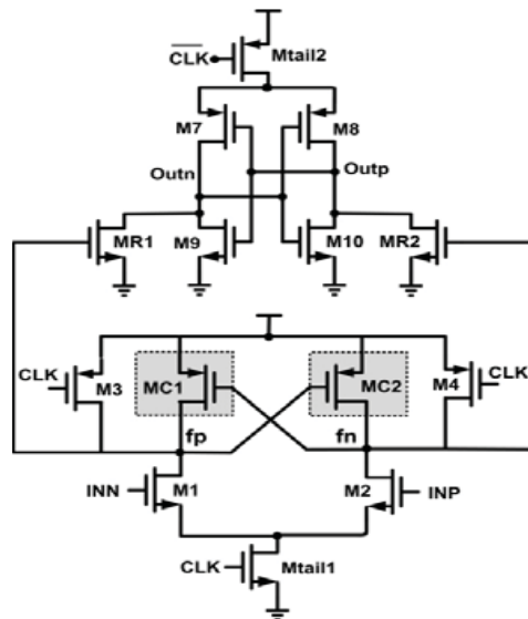
Fig. 5(a): Basic idea of the Proposed Comparator (Comparator 2)
