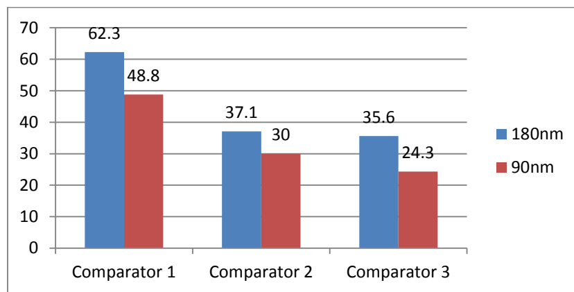
Fig. 15: Power consumption comparison of dynamic comparators
