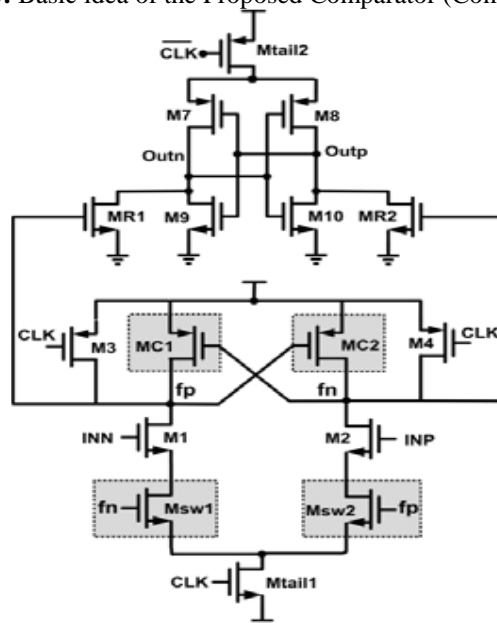
Fig. 5(b): Final Structure of the Proposed Comparator (Comparator 3)
