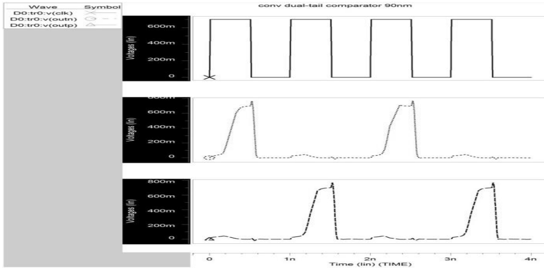
Fig. 12: Simulated Waveform of Comparator 1 (90nm)
