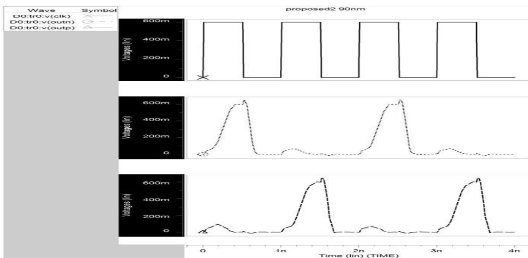
Fig. 14: Simulated Waveform of Comparator 3 (90nm)
