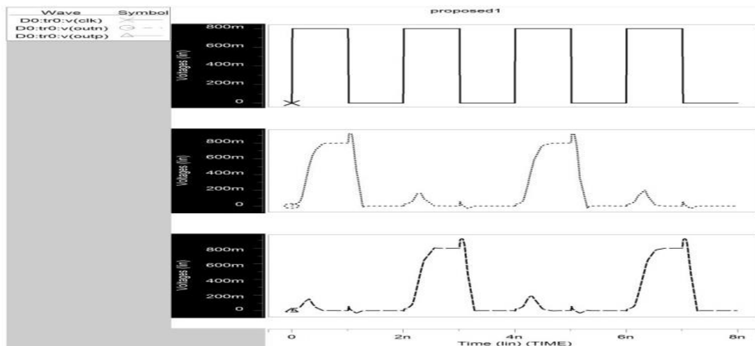
Fig. 10: Simulated Waveform of Comparator 2 (180nm)
