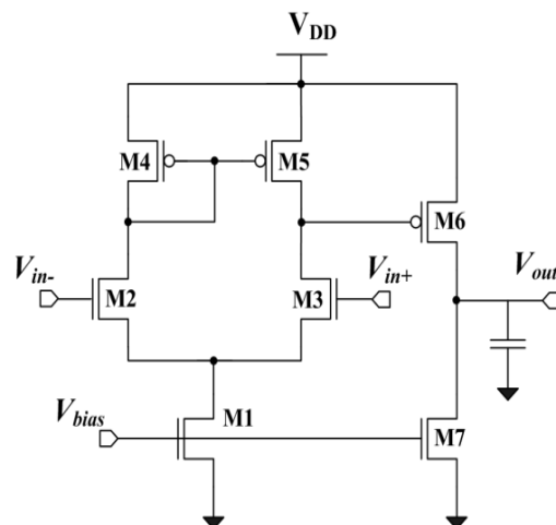
Fig. 2: Open-Loop Comparator
