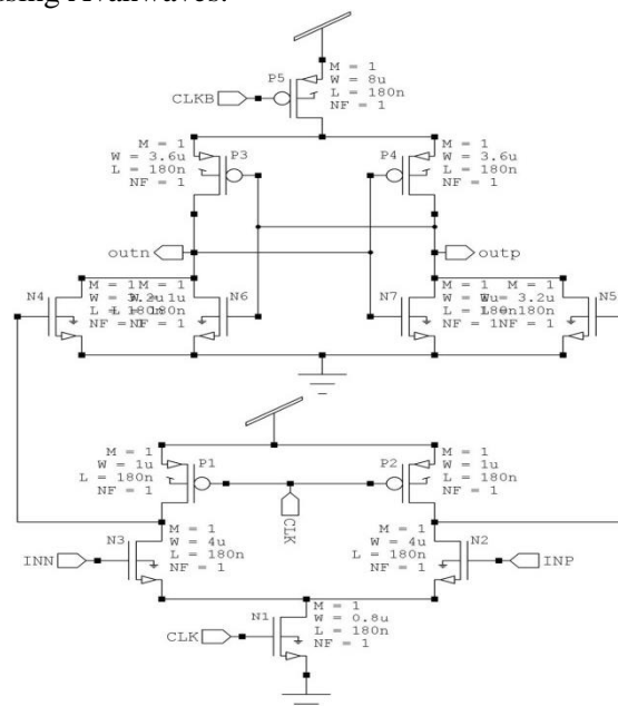
Fig. 6: Schematic of Conventional Dynamic Comparator (Comparator1)
