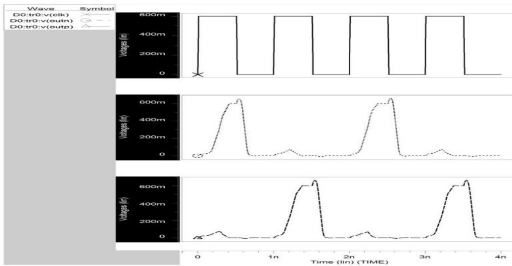
Fig. 13: Simulated Waveform of Comparator 2 (90nm)
