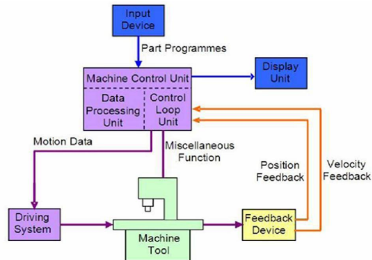
Figure 1. Block diagram of CNC machine.
