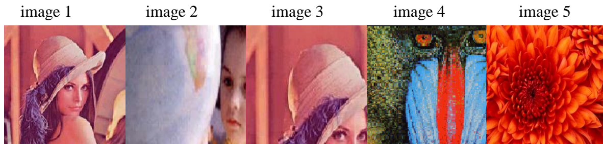
Figure.7 decompressed images
