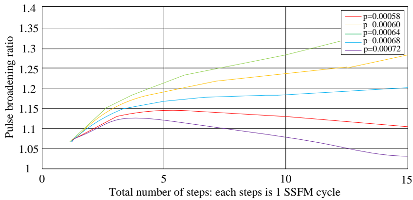
Figure 8. Pulse Broadening Ratio for different values of Power
