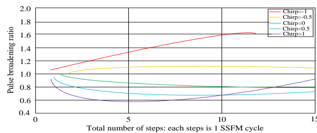
Figure 6. Pulse Broadening Ratio of Gaussian Pulse with different chirp
