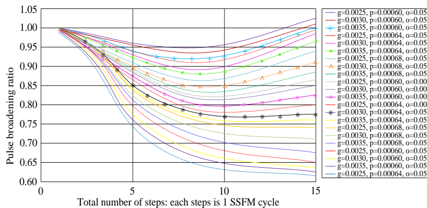
Figure 9. Pulse Broadening Ratio for different parameters
