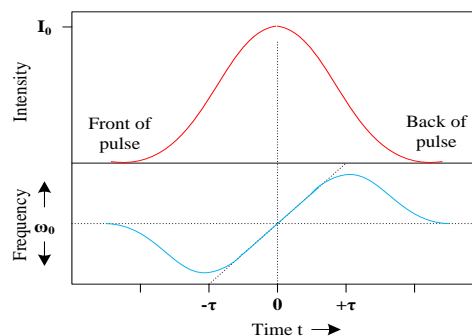
Figure 2. Self-phase modulation
