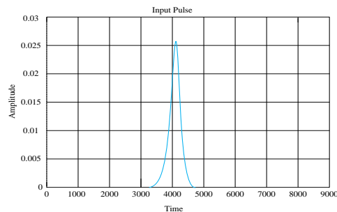
Figure 3. Gaussian Pulse
