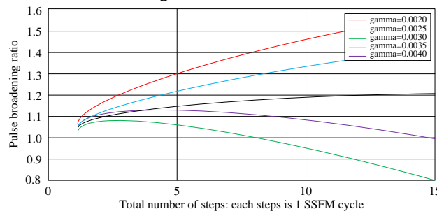
Figure 7. Pulse Broadening Ratio for different values of Nonlinearity
