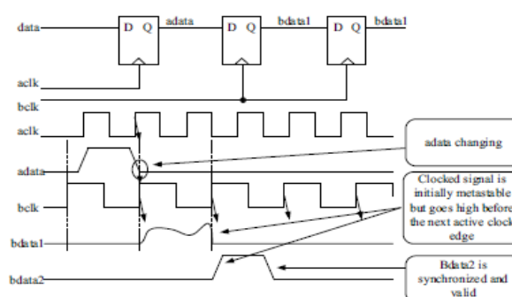
Figure (11): Two-flip-flop synchronizer
