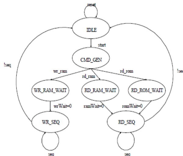
Figure (2): AHB Slave interface state machine
