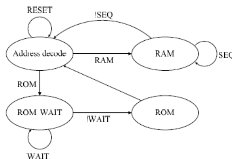
Figure (7): Sequential-access state machine
