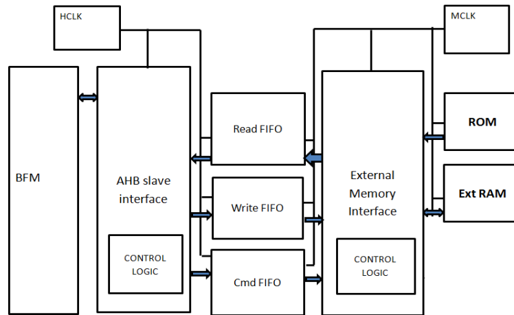
Figure (1): Architecture of AHB-MC
