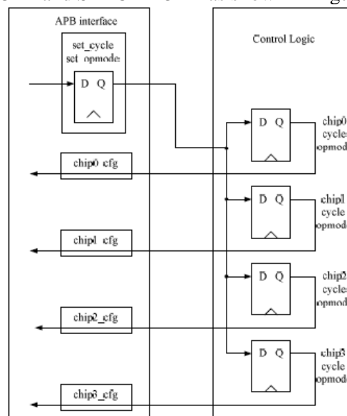
Figure (6): Chip configuration register
