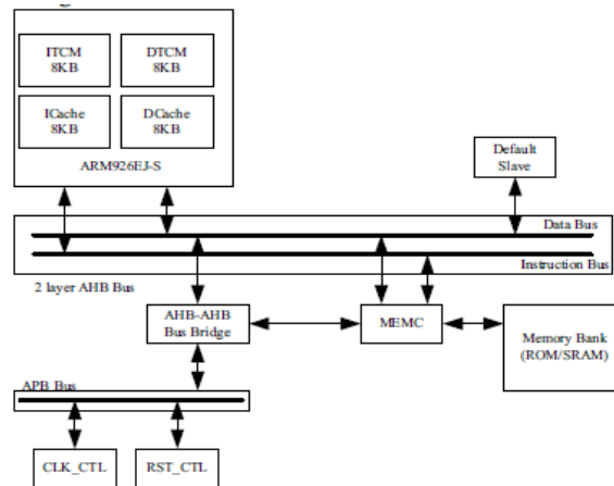
Figure (12): Minimum system for test
