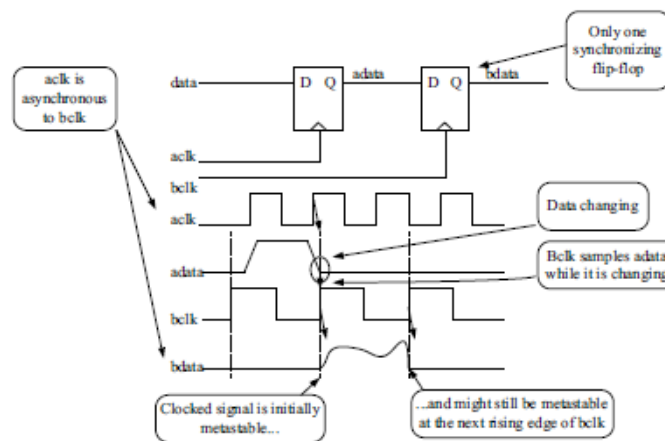
Figure (10): Asynchronous clocks and synchronization failure
