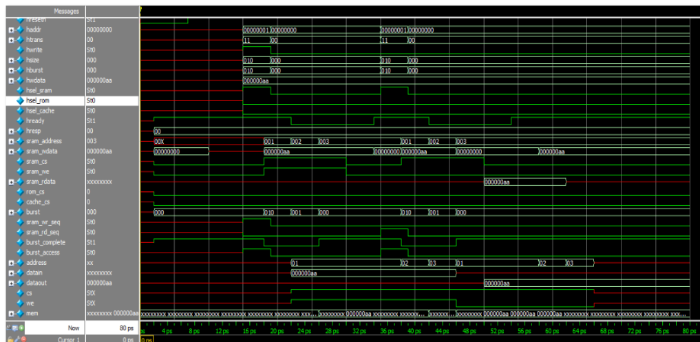
Figure (14): Write with zero wait state to RAM
