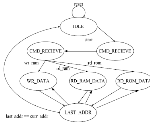
Figure (3): External Memory Interface State Machine
