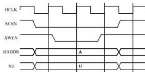
Figure (5): Memory write with two wait states
