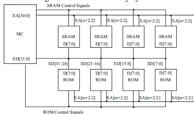
Figure (8): Memory system architecture
