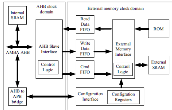
Figure (9): Clock domains
