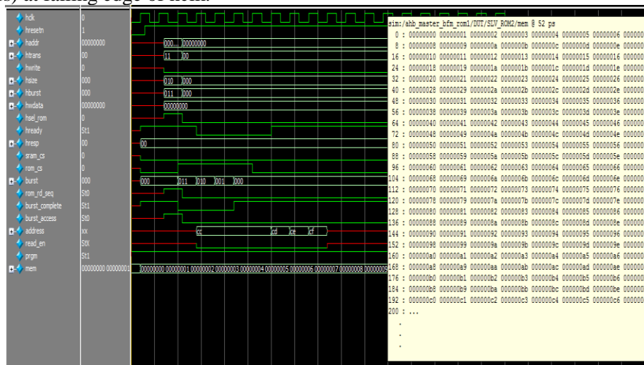
Figure (13): Read with zero wait state from ROM
