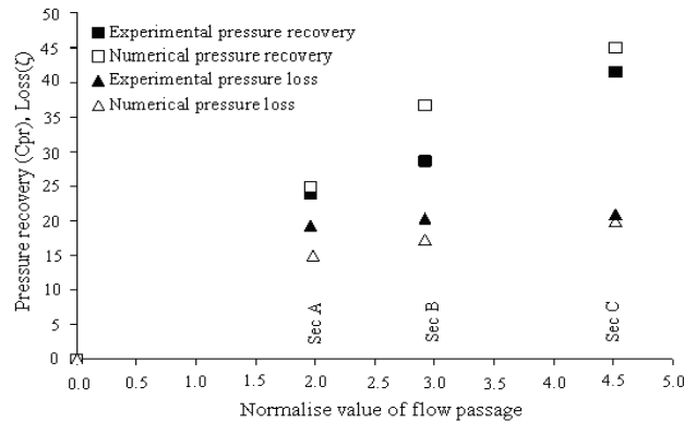
Figure 5: Comparison of performance parameters obtained through computational and experimental investigation
