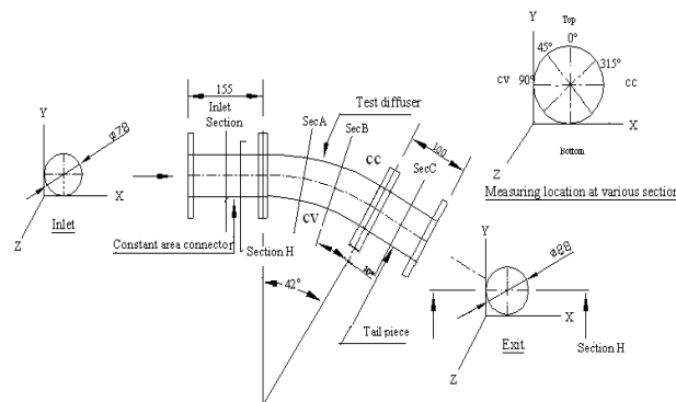
Figure 1: Geometry of test diffuser and measuring locations
