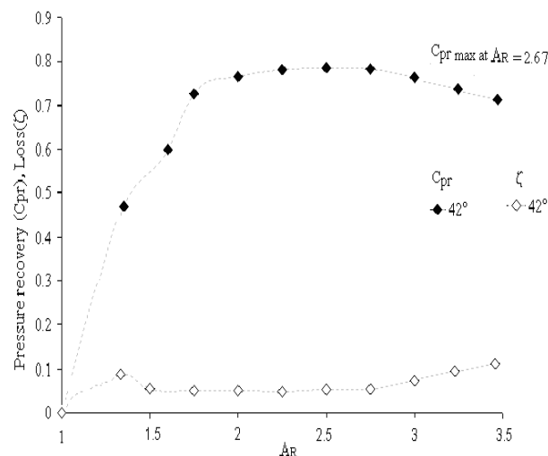
Figure 6: Variation of mass average pressure recovery and loss coefficients.
