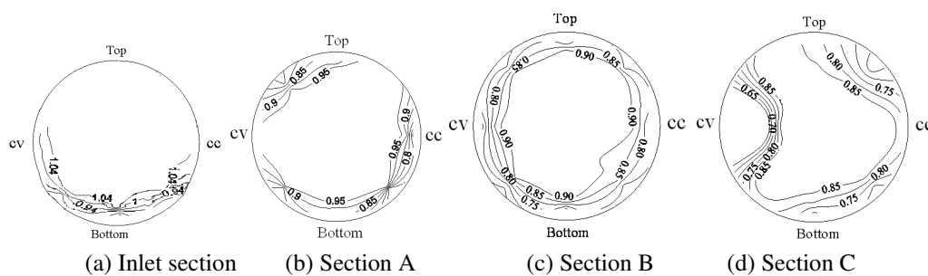
Figure 2: Mean velocity contour
