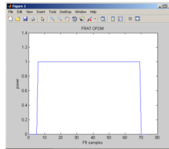
Fig. 10 FRAT OFDM power spectrum for N=64 , N_z=10
