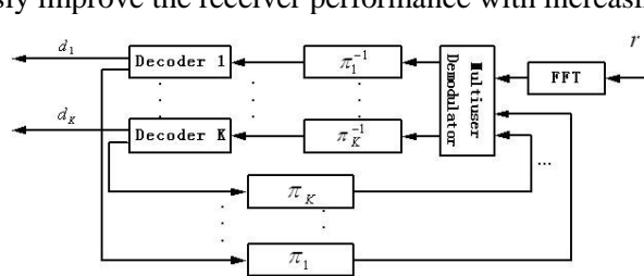
Fig. 6 Structure of iterative multi-user receiver
