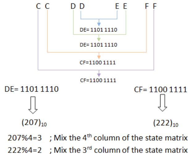
Fig. 5 Modified Mix Column
