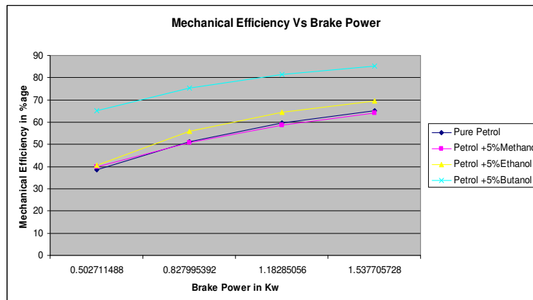
Figure 5 Mechanical Efficiency Vs Brake Power at various loads
