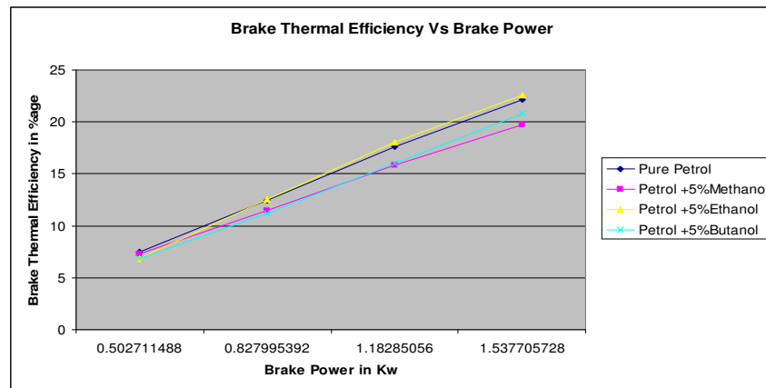
Figure 3 Brake Thermal Efficiency Vs Brake Power at various loads
