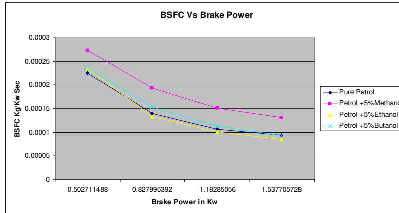
Figure 4 Specific Fuel Consumption (BSFC) Vs Brake Power at various loads
