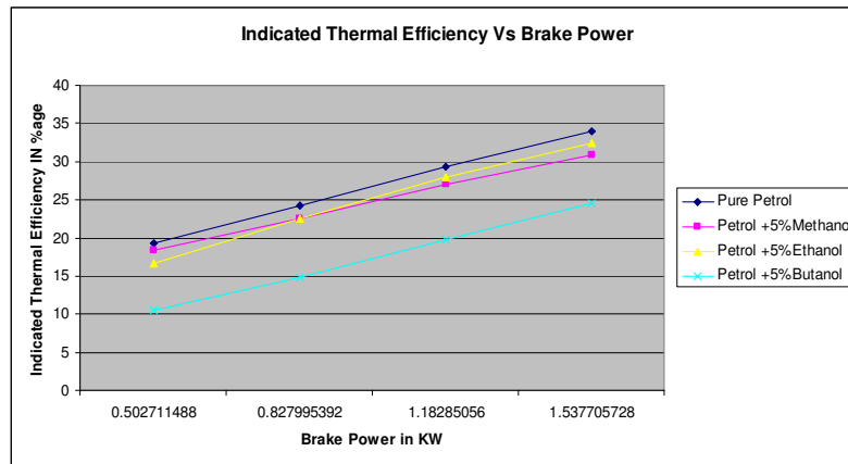
Figure 6. Indicated Thermal Efficiency Vs Brake Power at various loads
