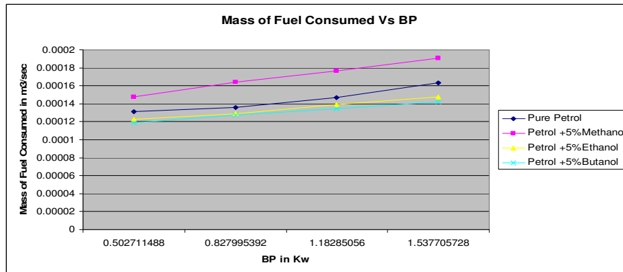
Figure 2 Fuel Consumption Vs Brake Power at various loads
