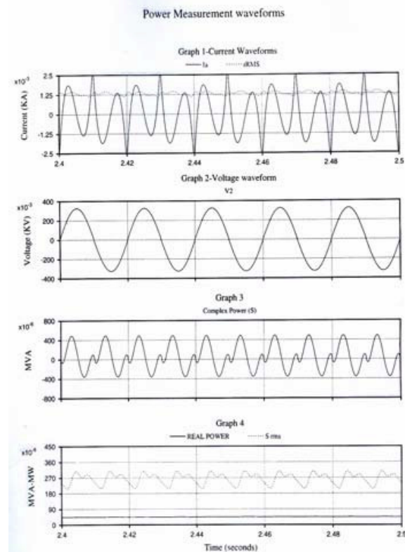
Fig. 3: Leading mode waveforms, V_{d.c.}=250 V
