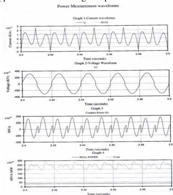
Fig. 5: Leading mode waveforms, harmonics injection in grid voltage V_2 ; V_{d.c.}=250 V
