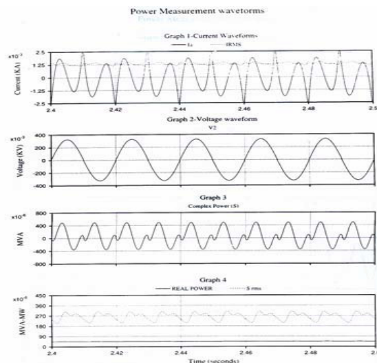
Fig. 4: Leading mode waveforms for V_{d.c.}=250V
