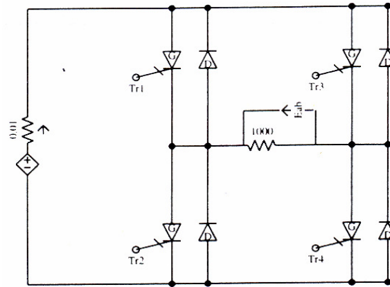
Fig. 1: The inverter circuit
