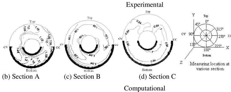
FIGURE 4. Comparison of normalized velocity distribution at Section A, Section B and Section C obtained through Computational and Experimental investigation
