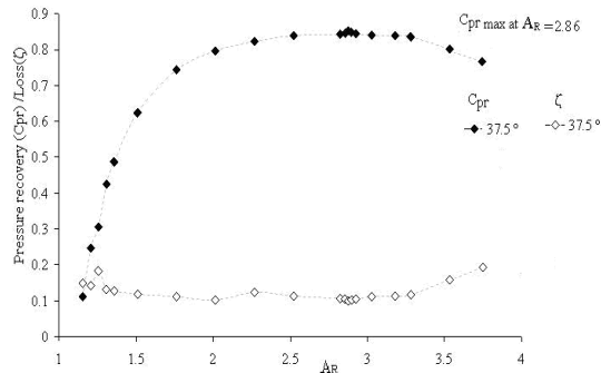
FIGURE 6. Variation of mass average pressure recovery and loss coefficients.
