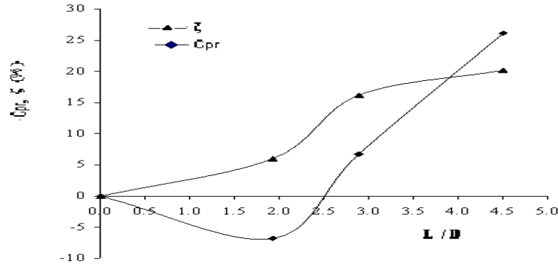
FIGURE 3. Variation of mass average pressure recovery and loss coefficients
