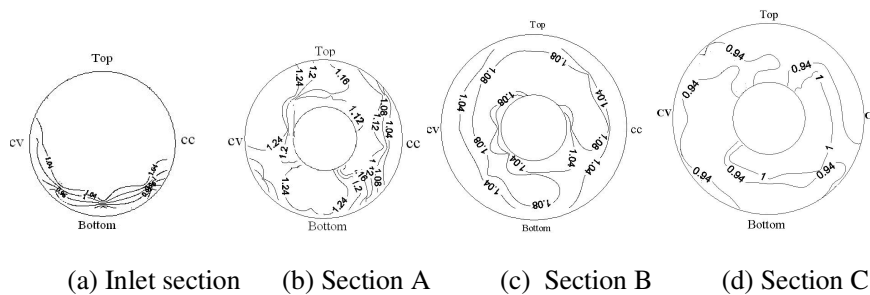
FIGURE 2. Mean velocity Contour
