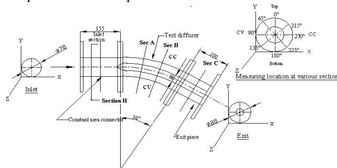
FIGURE 1. Geometry of test diffuser and measuring locations
