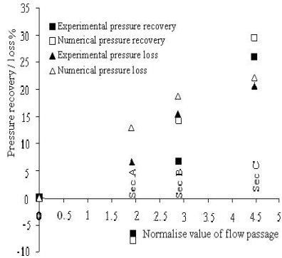
FIGURE 5. Comparison of Performance parameters obtained through computational and experimental investigation
